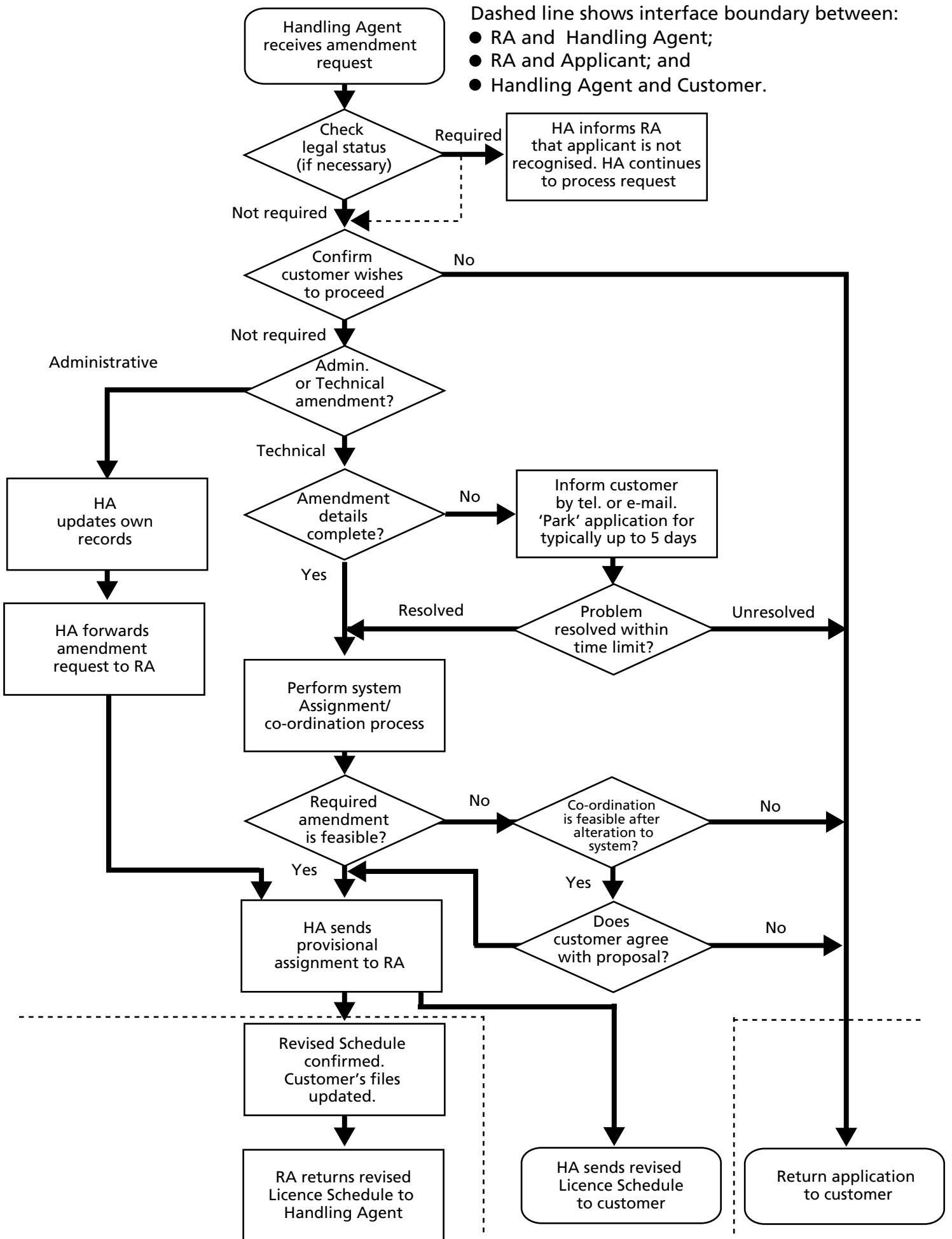
Figure I.1: SCANNING TELEMETRY LICENCE AMENDMENT PROCESS
