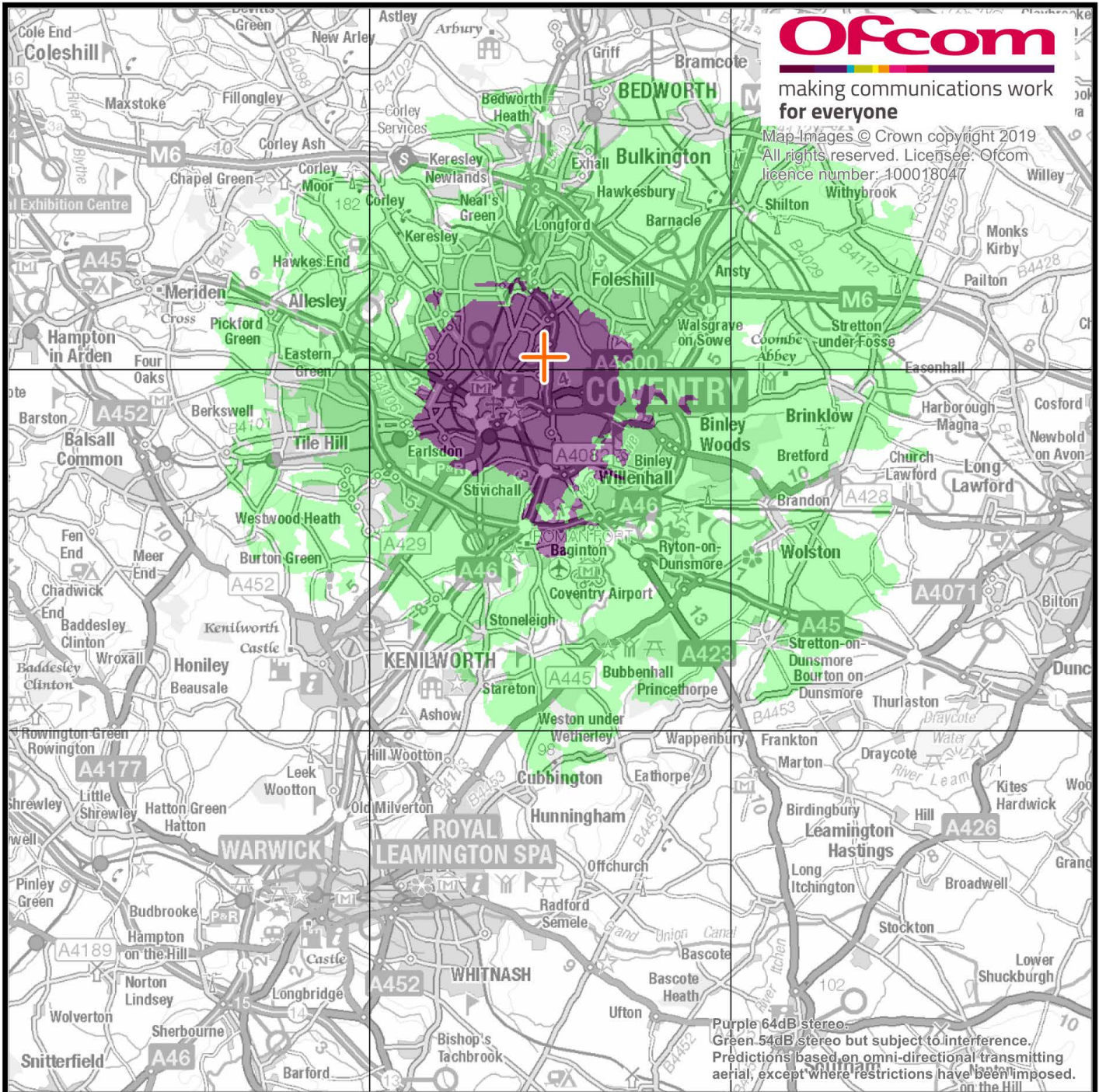
Coventry (The Hillz FM) community radio coverage area - 22nd August 2019
