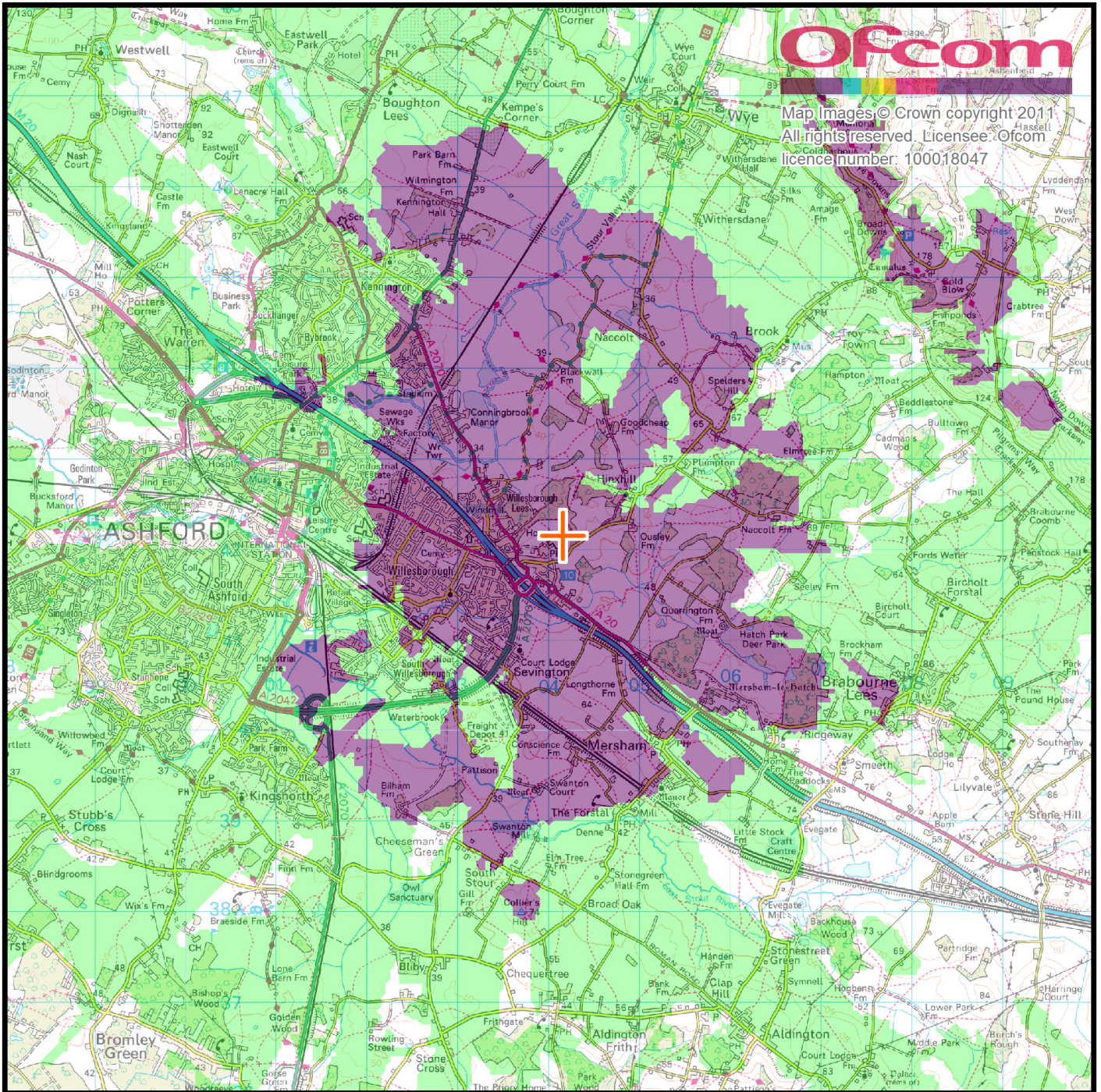
Ashford (AHBS) community radio coverage area - 21st April 2011
