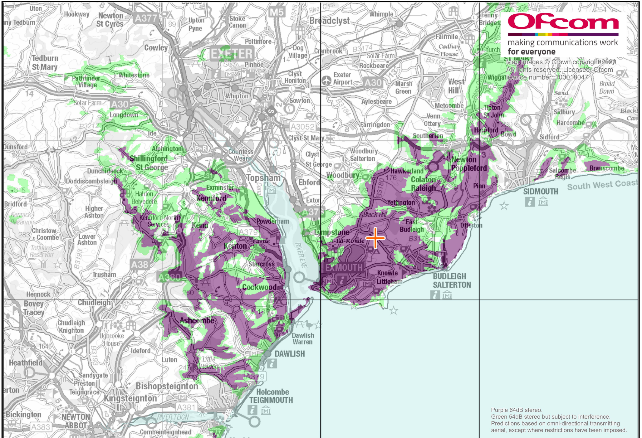
Exmouth (ExmouthAiR) community radio coverage area - 20th February 2019
