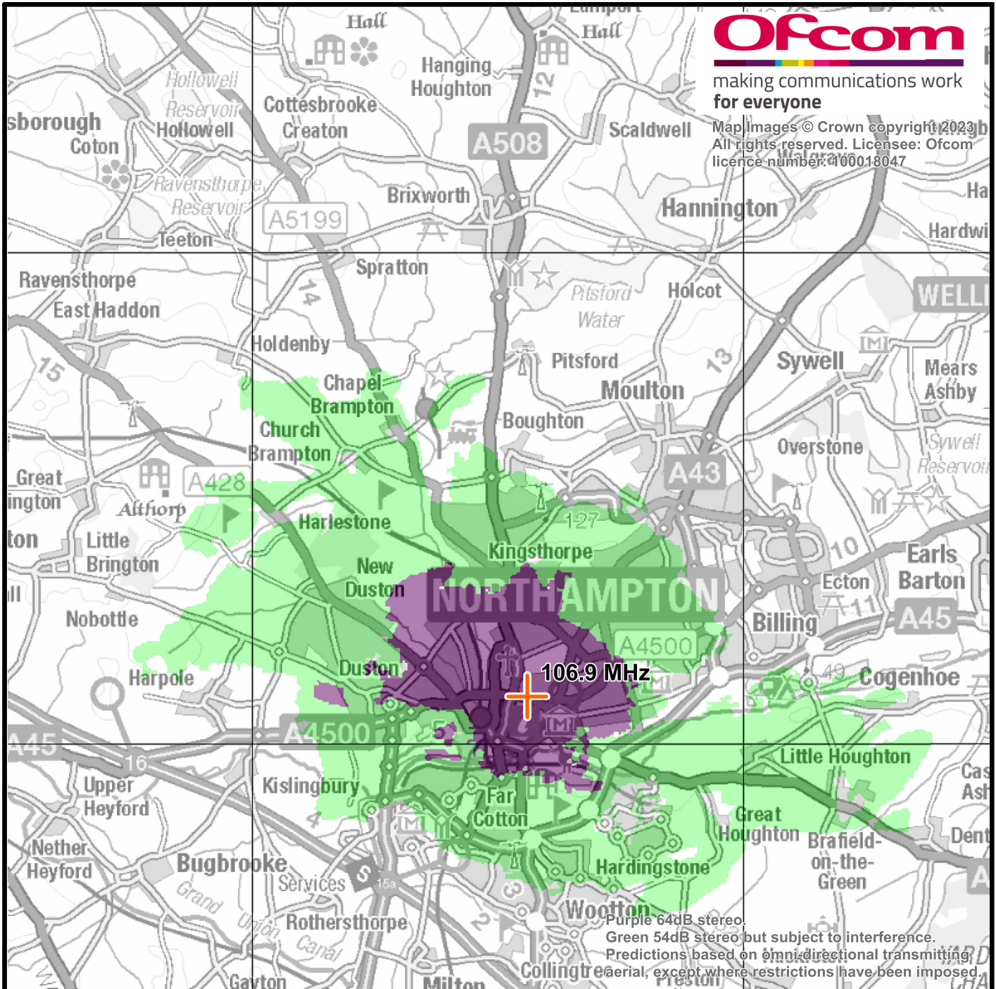
Northampton (NLive) community radio coverage area - 15th November 2022
