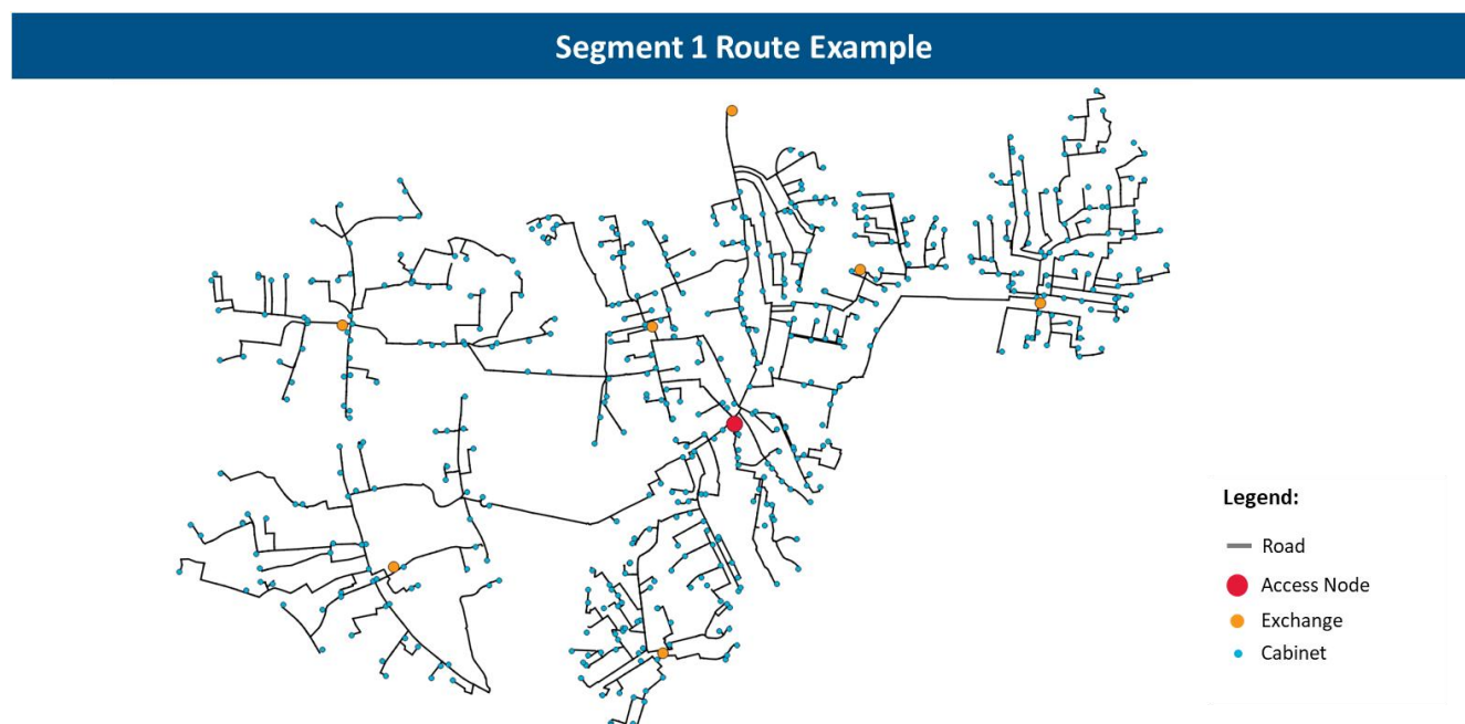
Figure 14. Example of Segment 1 Routing
