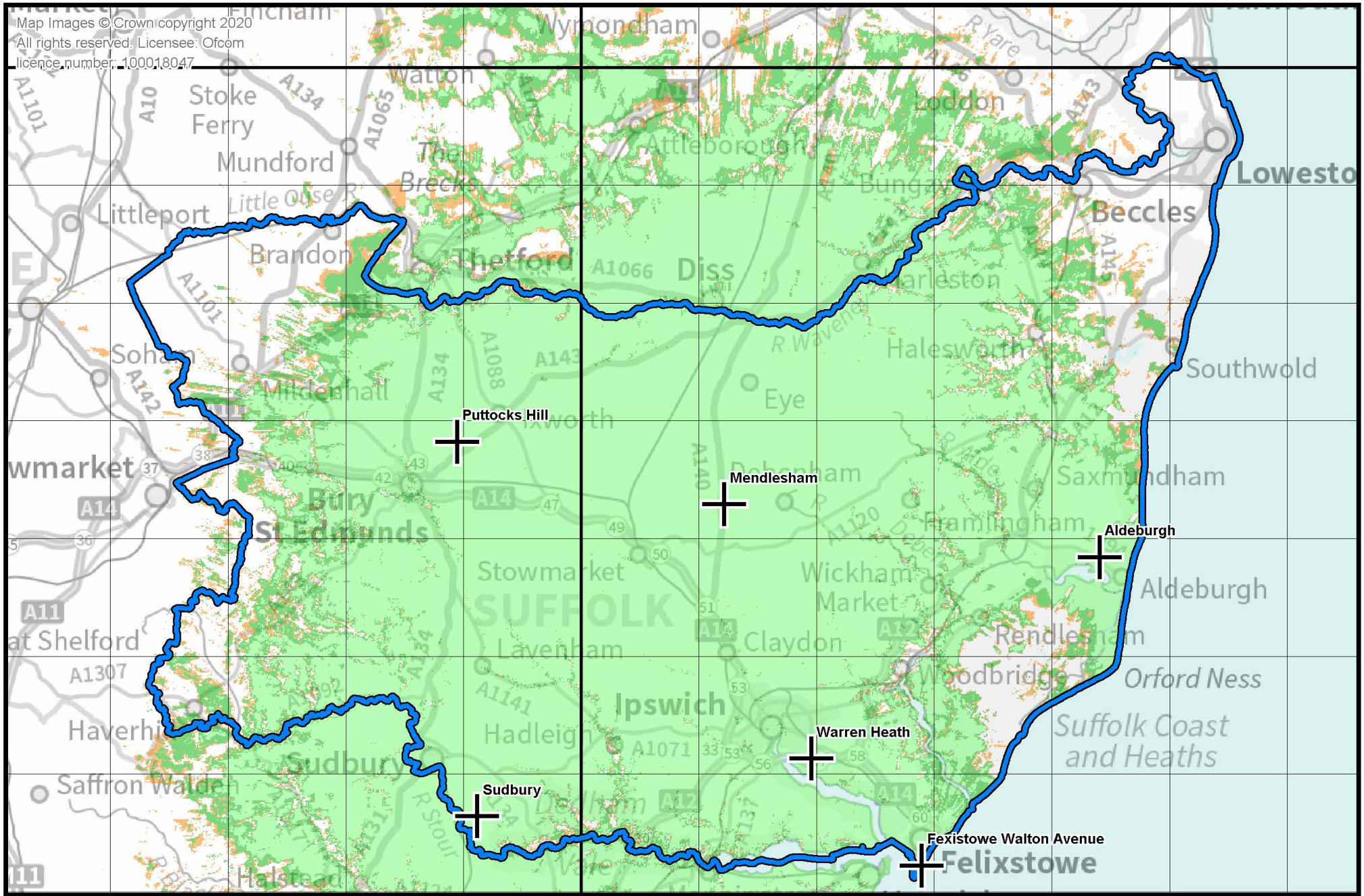
Suffolk local DAB multiplex service Predicted indoor coverage normal propagation conditions, Final
