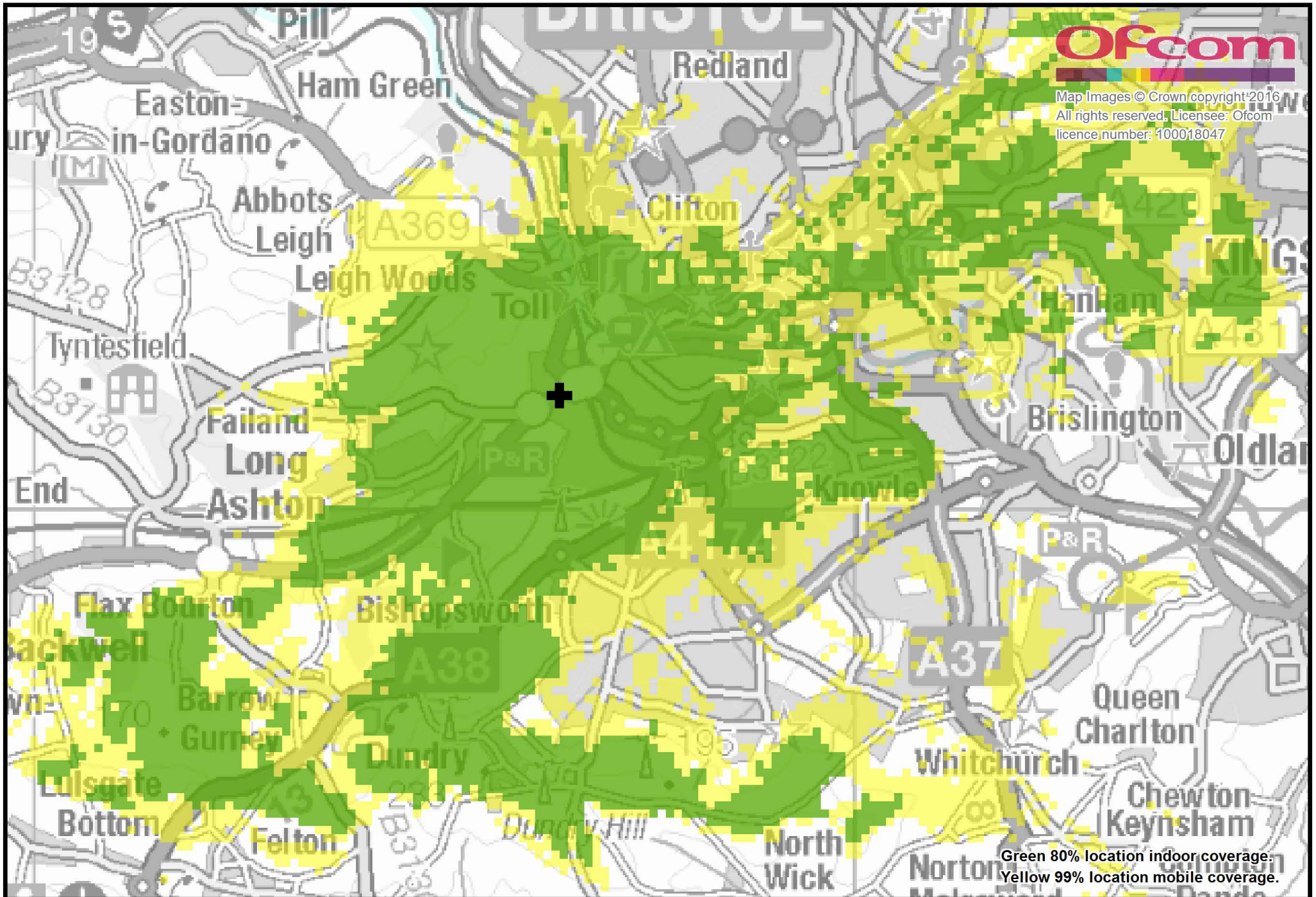
Bristol small scale DAB trial predicted coverage. April 2016.
