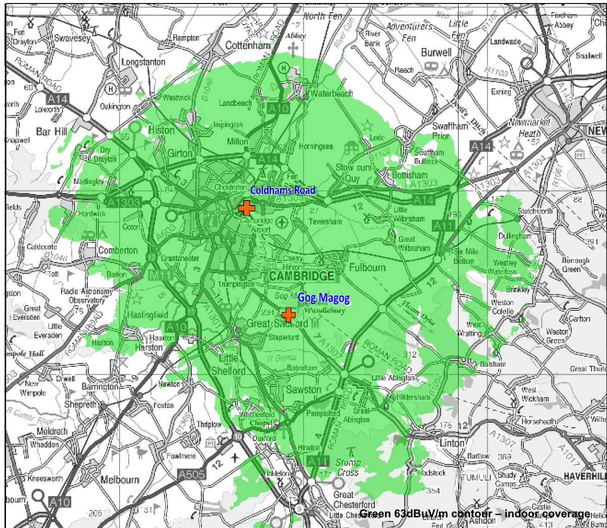
Figure 1. Predicted indoor coverage of the Cambridge small-scale DAB multiplex, January 2023
