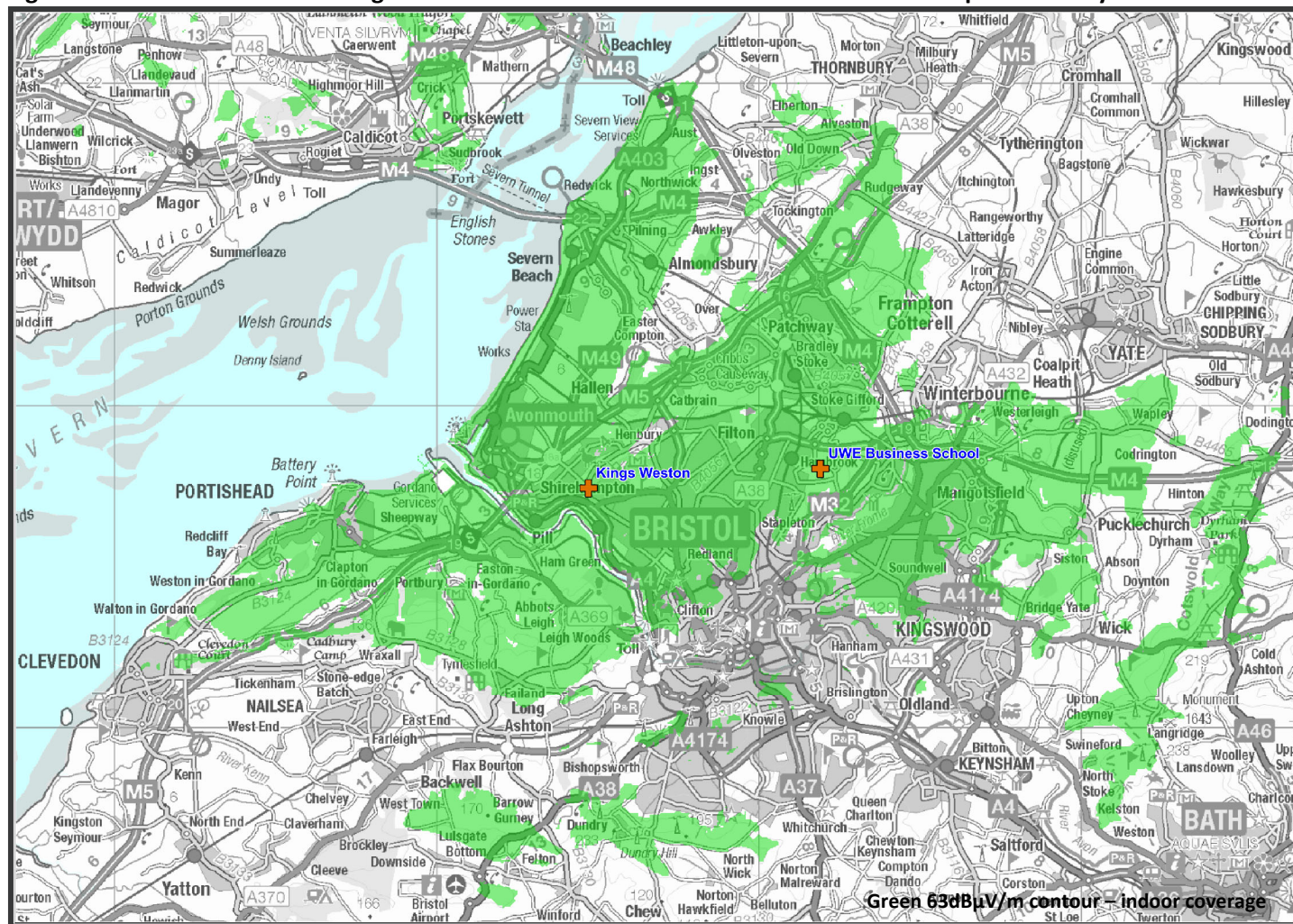
Figure 1: Predicted indoor coverage of the Avonmouth and Filton small-scale DAB multiplex. January 2023
