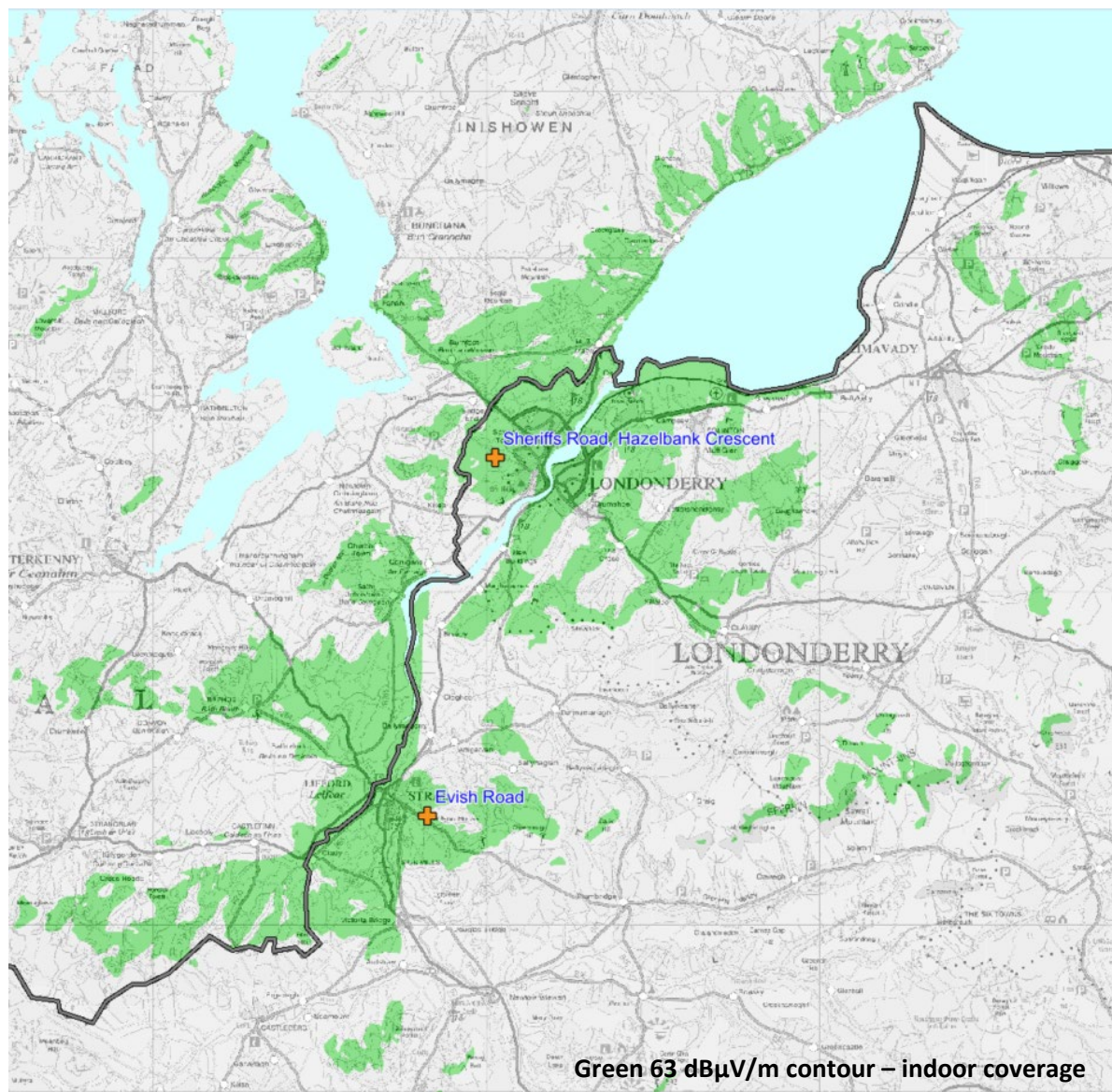
Figure 1: Predicted indoor coverage of the Derry / Londonderry small-scale DAB multiplex. January 2023
