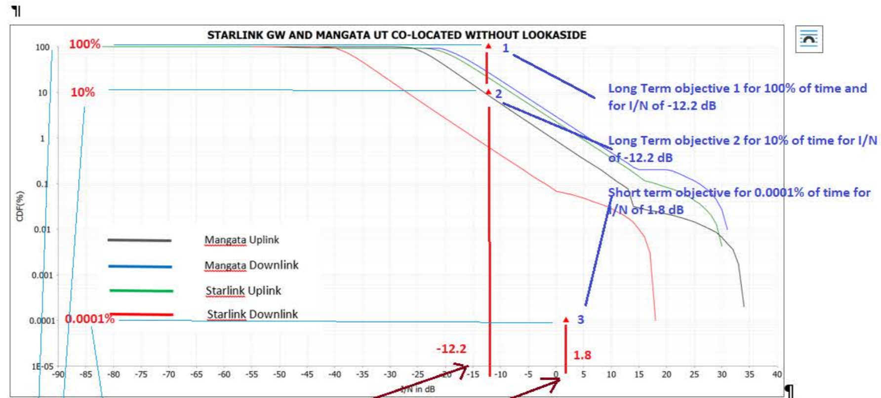
Figure 5: Starlink GW and Mangata UT collocated without lookaside
