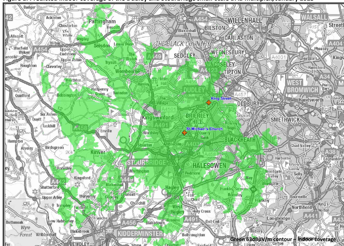
Figure 1: Predicted indoor coverage of the Dudley and Stourbridge small-scale DAB multiplex, January 2023
