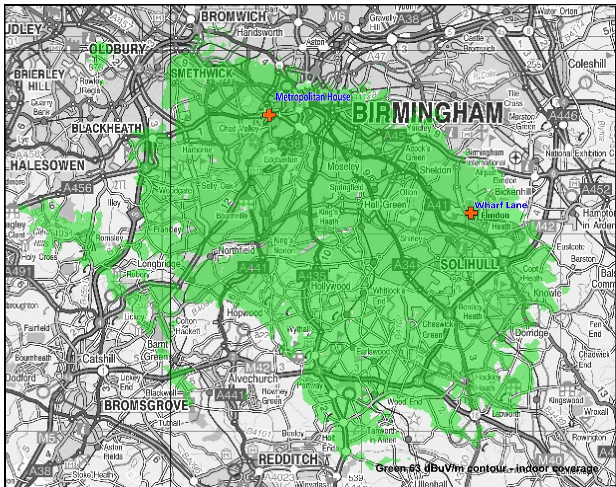
Figure 1. Predicted indoor coverage of the South Birmingham small-scale DAB multiplex, January 2023
