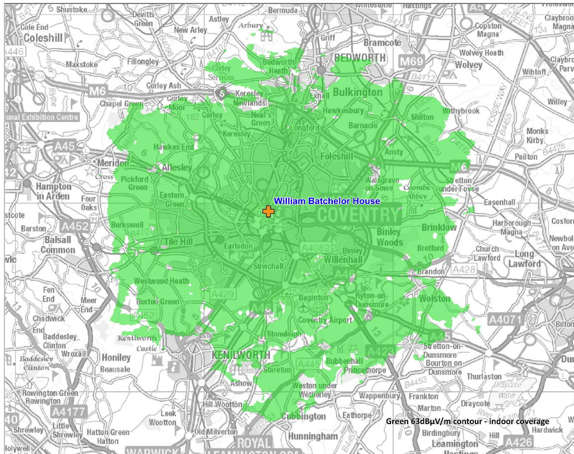
Figure 1. Predicted indoor coverage of the Coventry small-scale DAB multiplex, January 2023
