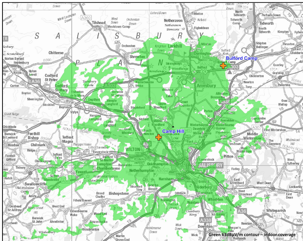
Figure 1. Predicted indoor coverage of the Salisbury small-scale DAB multiplex, January 2023
