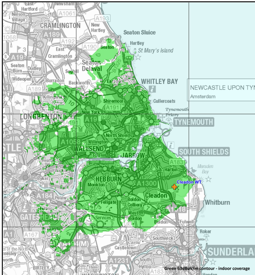
Figure 1. Predicted indoor coverage of the Tynemouth & South Shields small-scale DAB multiplex, January 2023
