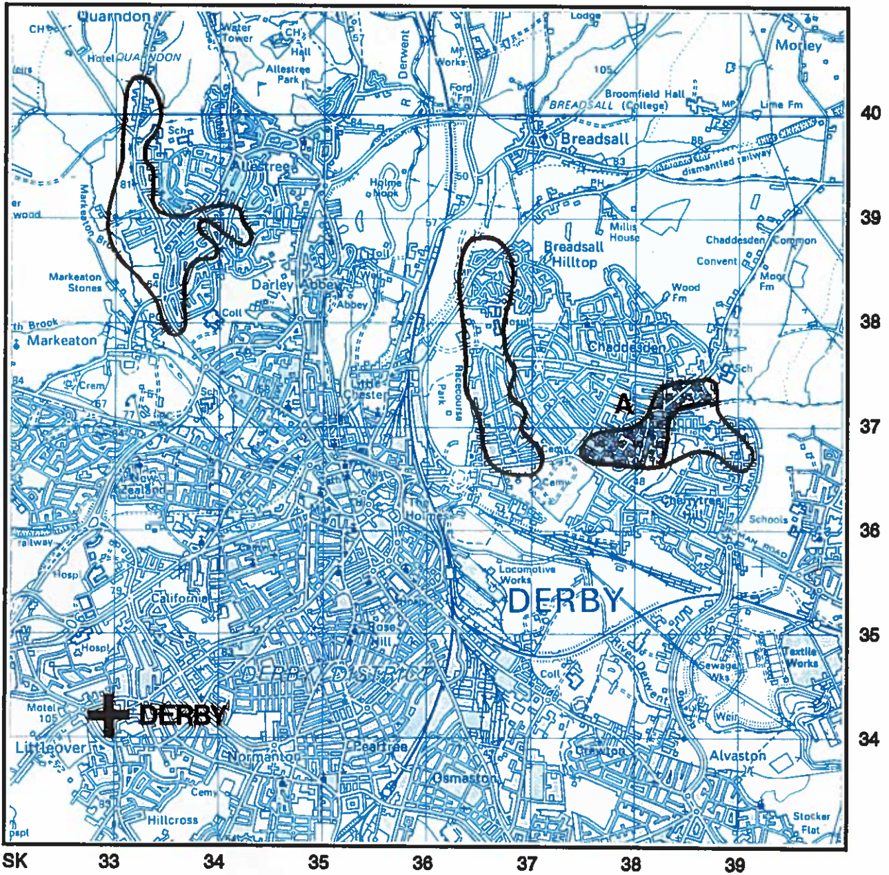
FIGURE 1 11102 DERBY UHF RELAY STATION COVERAGE ( FROM SITE TEST )
