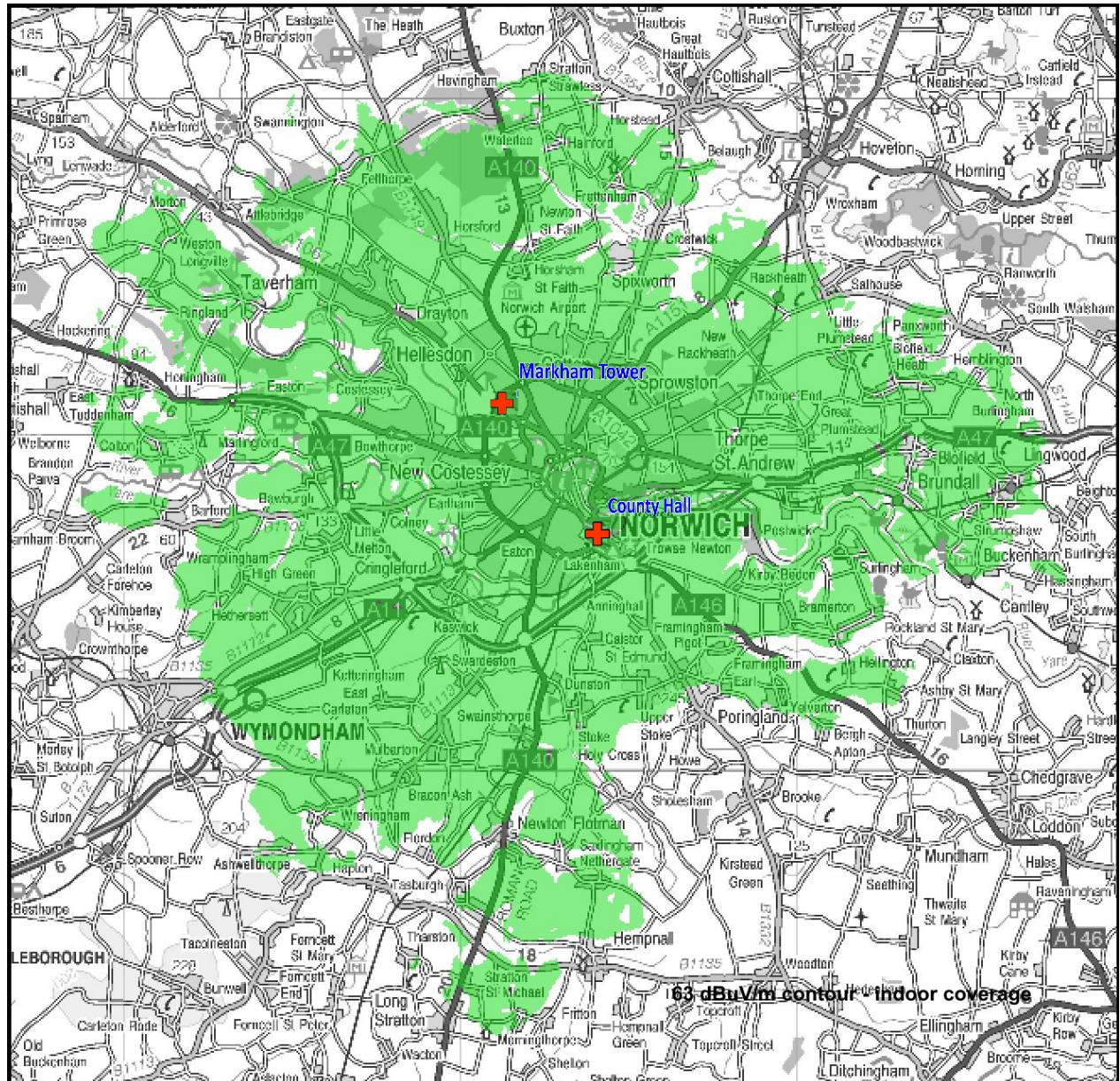
Figure 1. Predicted indoor coverage of the Norwich small-scale DAB multiplex, January 2023
