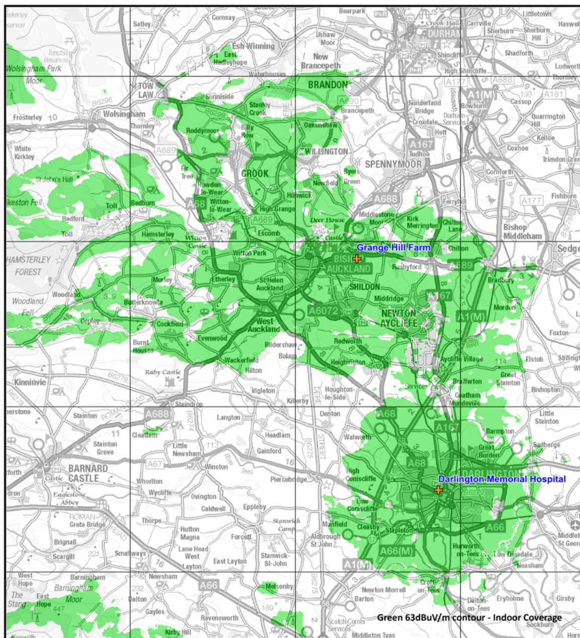
Figure 1: Predicted indoor coverage of the Darlington & Bishop Auckland small-scale DAB multiplex. July 2023
