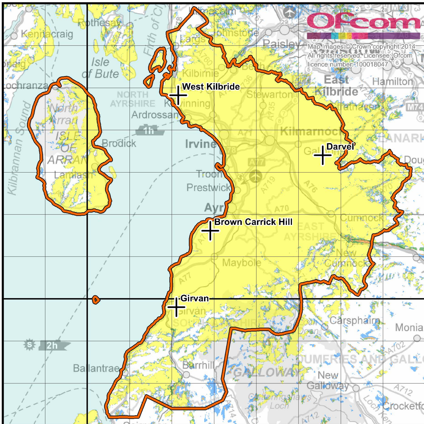
Ayrshire local DAB multiplex service Mobile coverage enhanced propagation conditions, Final
