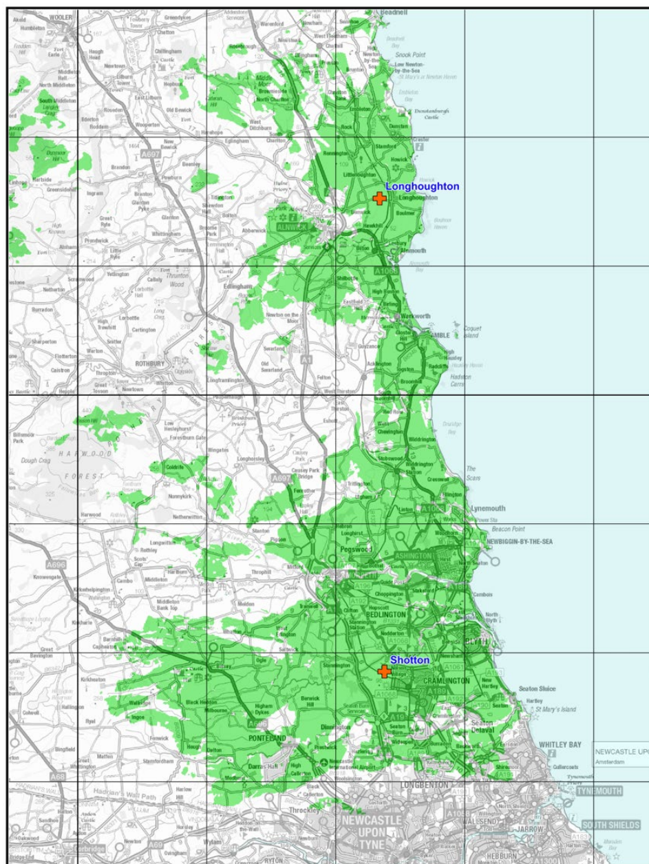
Figure 1: Predicted indoor coverage of the Alnwick and Morpeth small-scale DAB multiplex. February 2025
