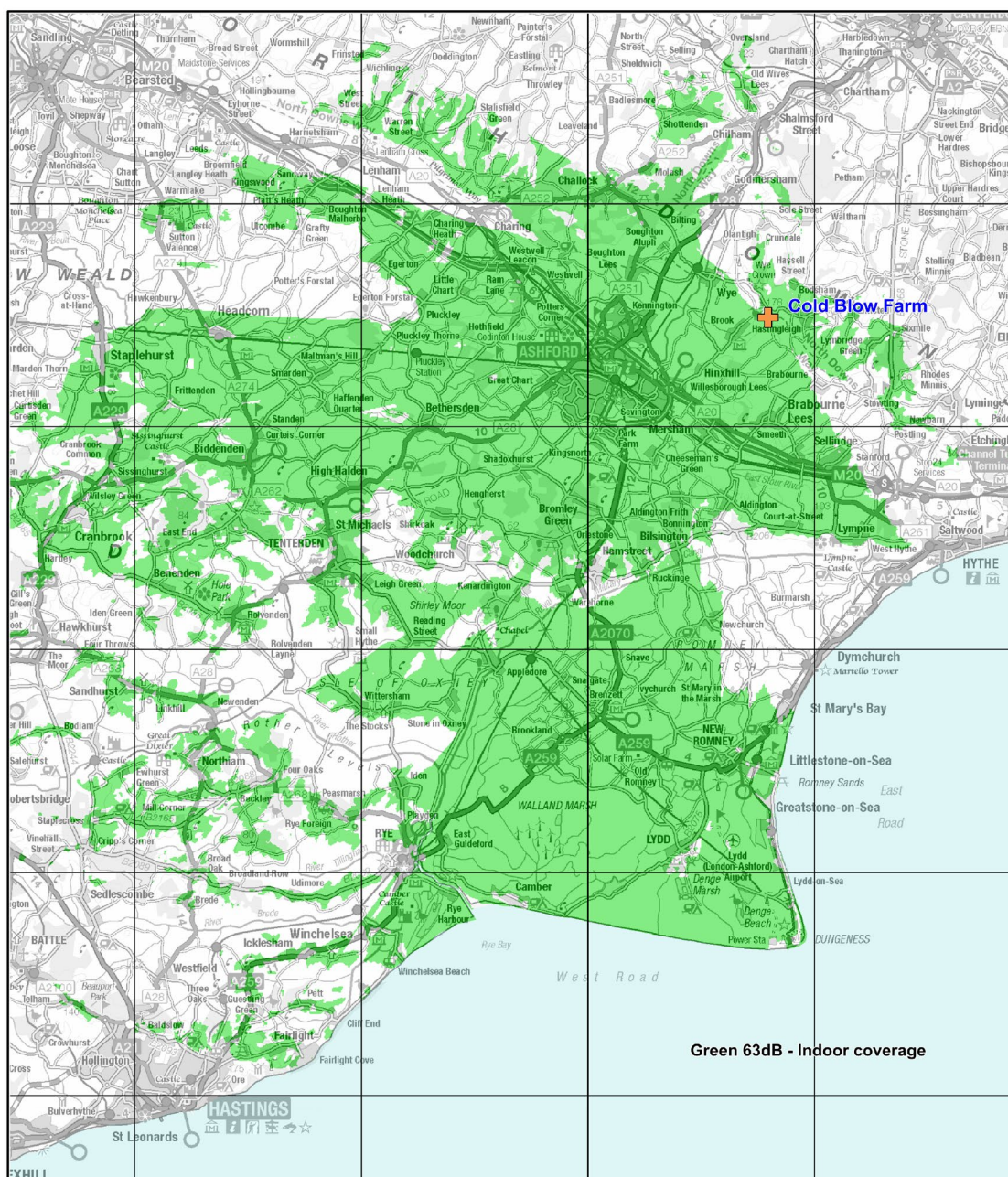
Figure 1: Predicted indoor coverage of the Ashford & Dungeness small-scale DAB multiplex. January 2026
