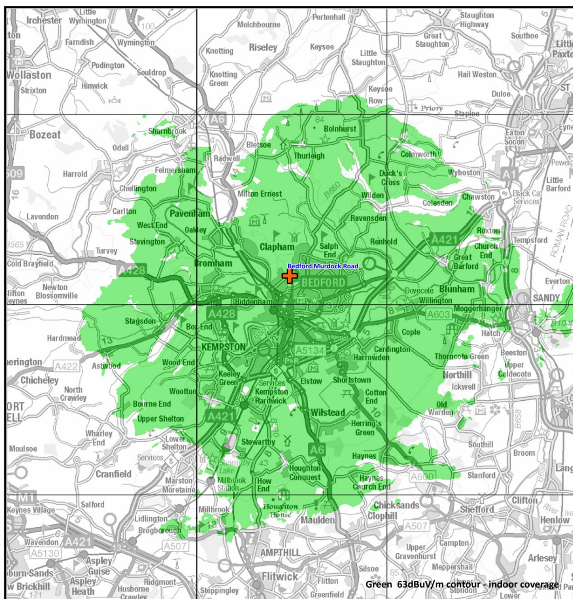
Figure 1: Predicted indoor coverage of the Bedford small-scale DAB multiplex. March 2024
