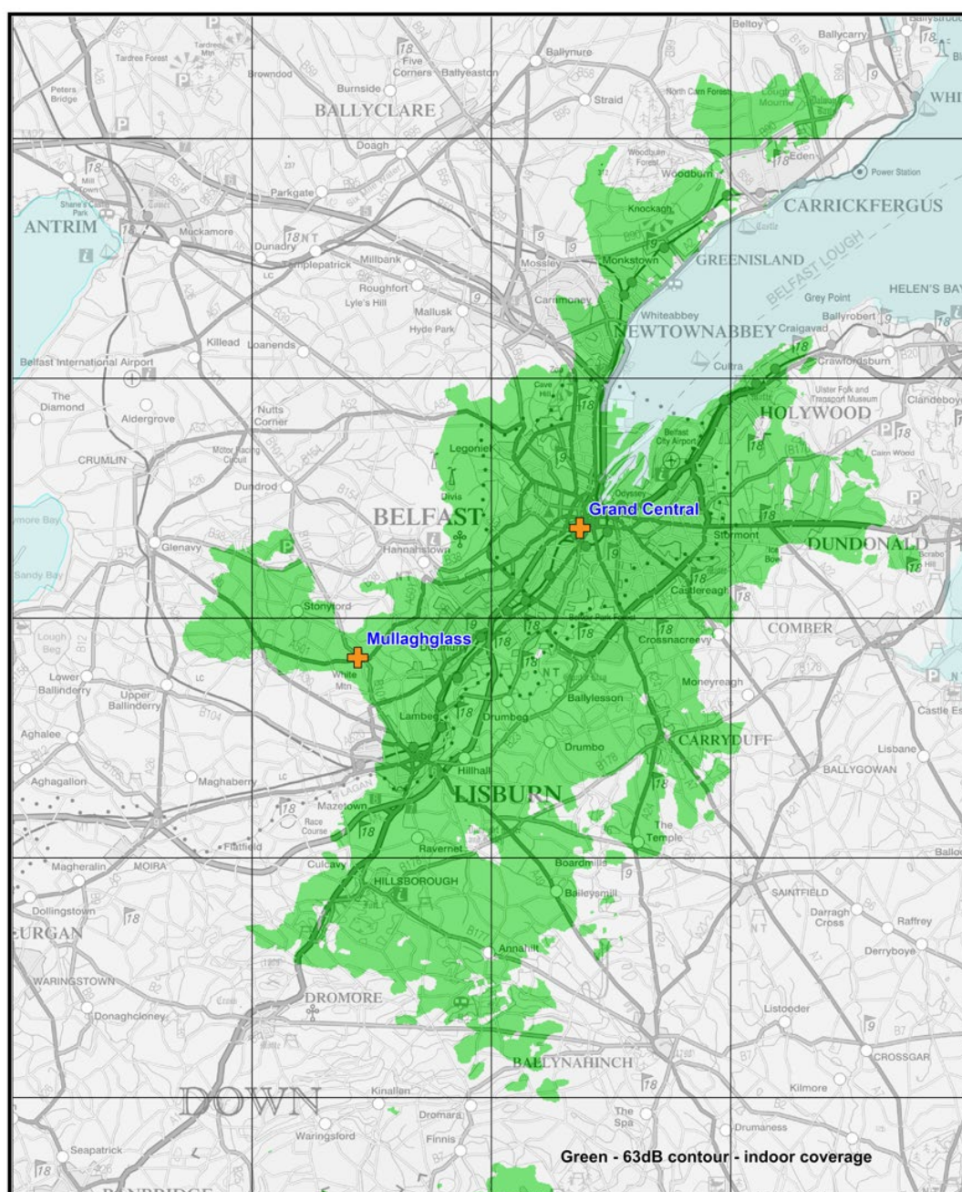
Figure 1: Predicted indoor coverage of the Belfast & Lisburn small scale DAB multiplex. January 2024
