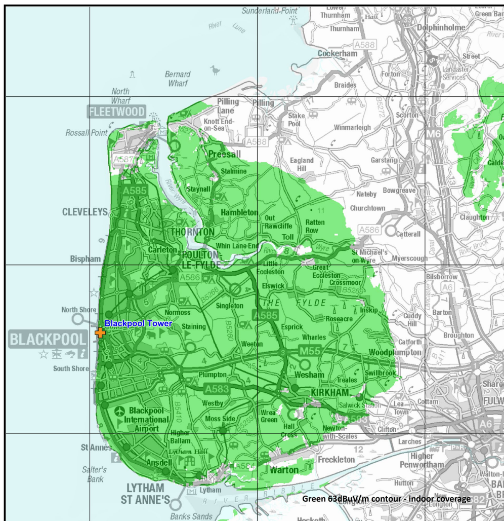
Figure 1: Predicted indoor coverage of the Blackpool small-scale DAB multiplex, March 2023
