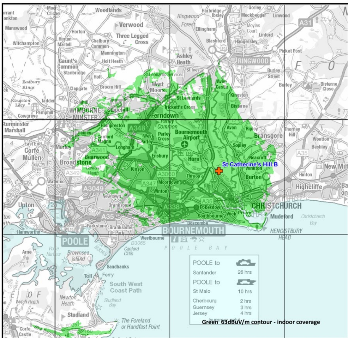
Figure 1: Predicted indoor coverage of the Bournemouth and Boscombe small-scale DAB multiplex. January 2026
