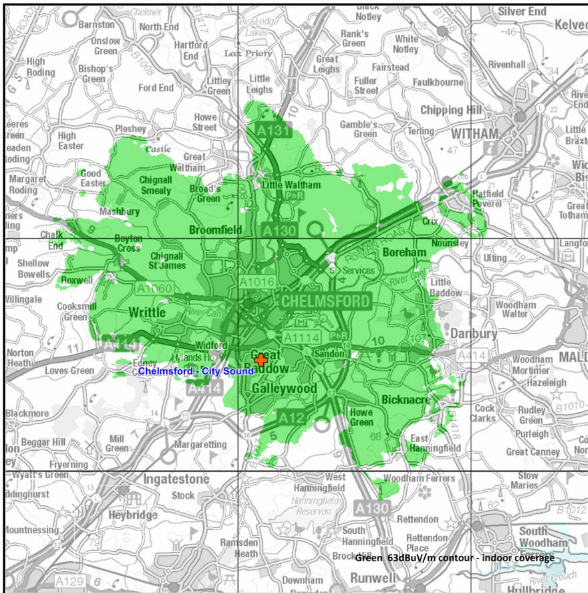
Figure 1: Predicted indoor coverage of the Chelmsford small-scale DAB multiplex. January 2026
