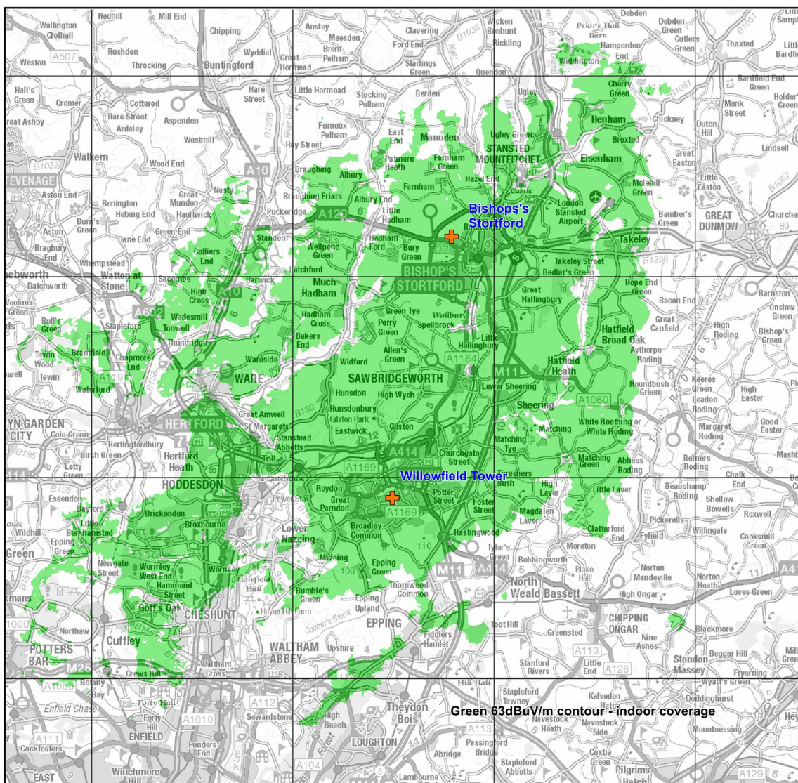
Figure 1: Predicted indoor coverage of the Harlow small-scale DAB multiplex. January 2026.
