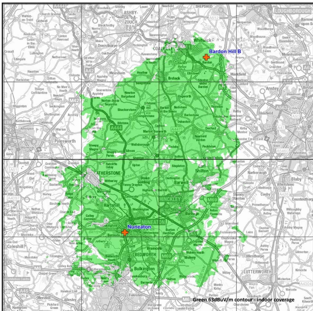
Figure 1: Predicted indoor coverage of the Hinckley and Nuneaton small-scale DAB multiplex. September 2022
