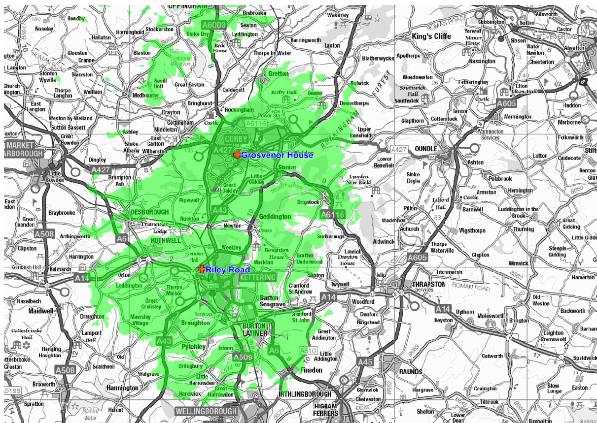
Figure 1: Predicted indoor coverage of the Kettering and Corby small-scale DAB multiplex. May 2026
