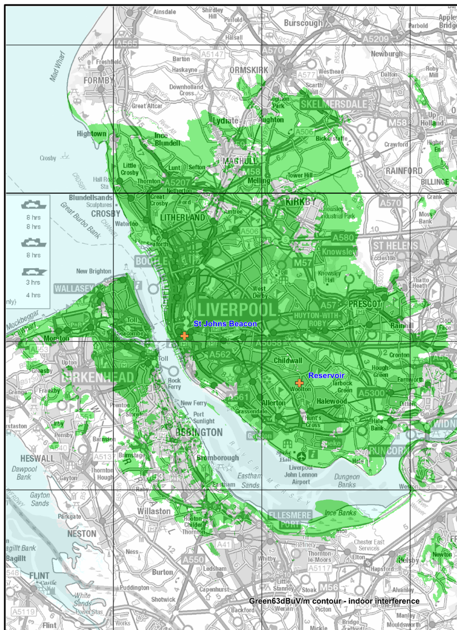
Figure 1: Predicted indoor coverage of the Liverpool small-scale DAB multiplex. July 2024.
