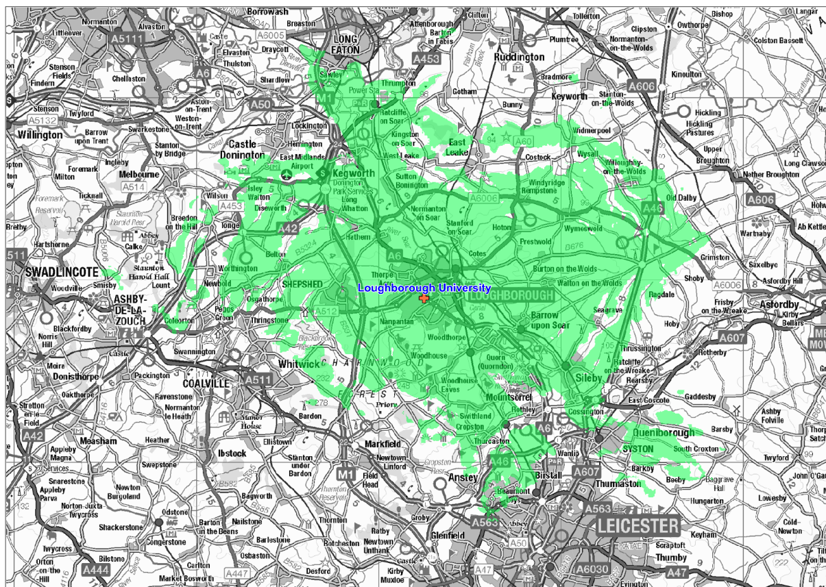
Figure 1: Predicted indoor coverage of the Loughborough small-scale DAB multiplex. July 2025
