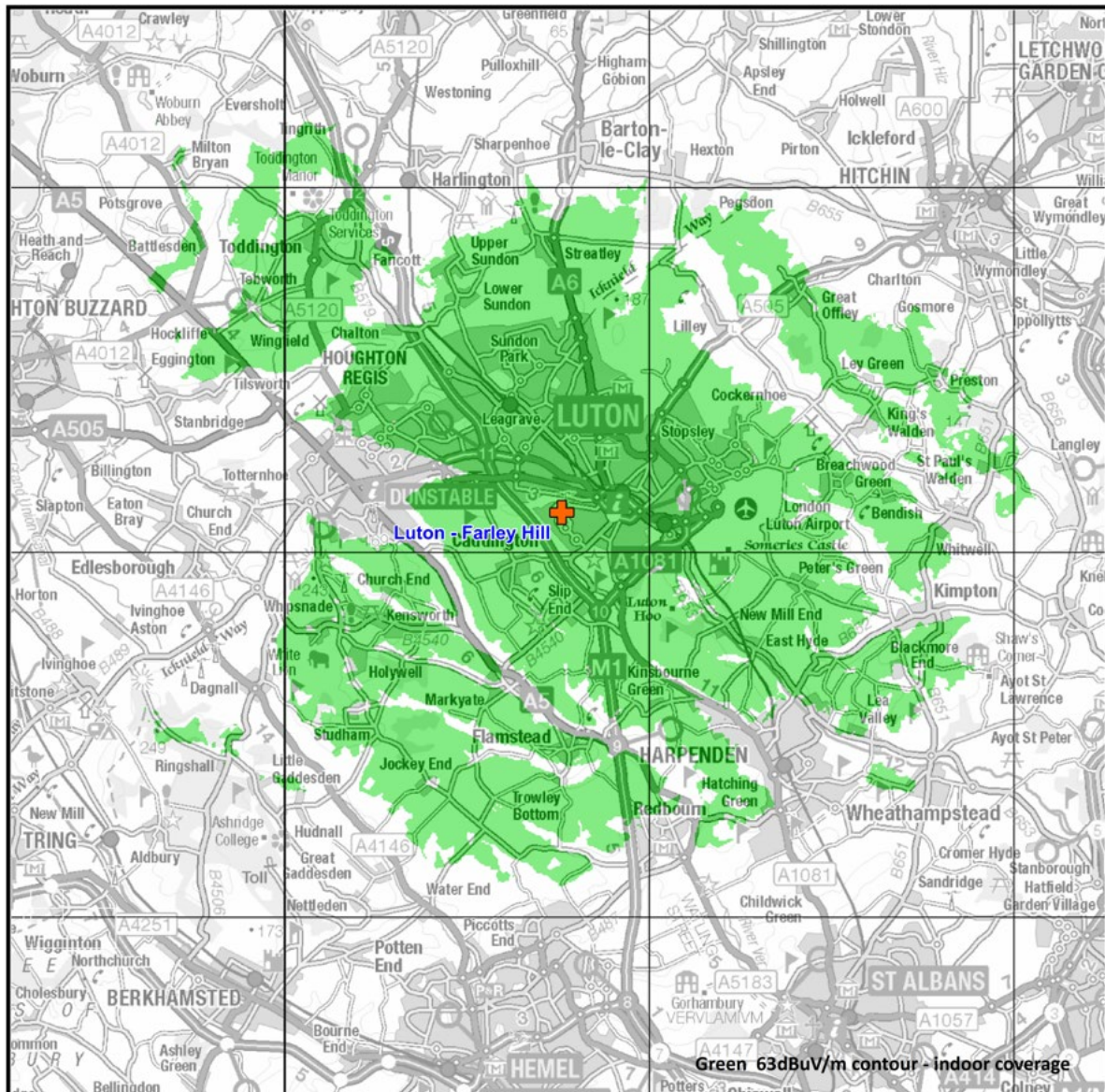
Figure 1: Predicted indoor coverage of the Luton small-scale DAB multiplex. January 2026
