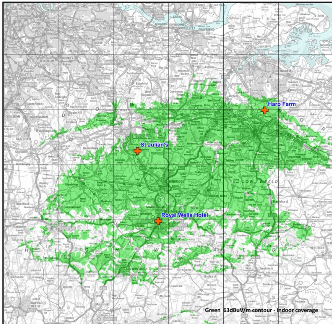
Figure 1: Predicted indoor coverage of the Maidstone Tonbridge & Tunbridge Wells small-scale DAB multiplex. January 2026
