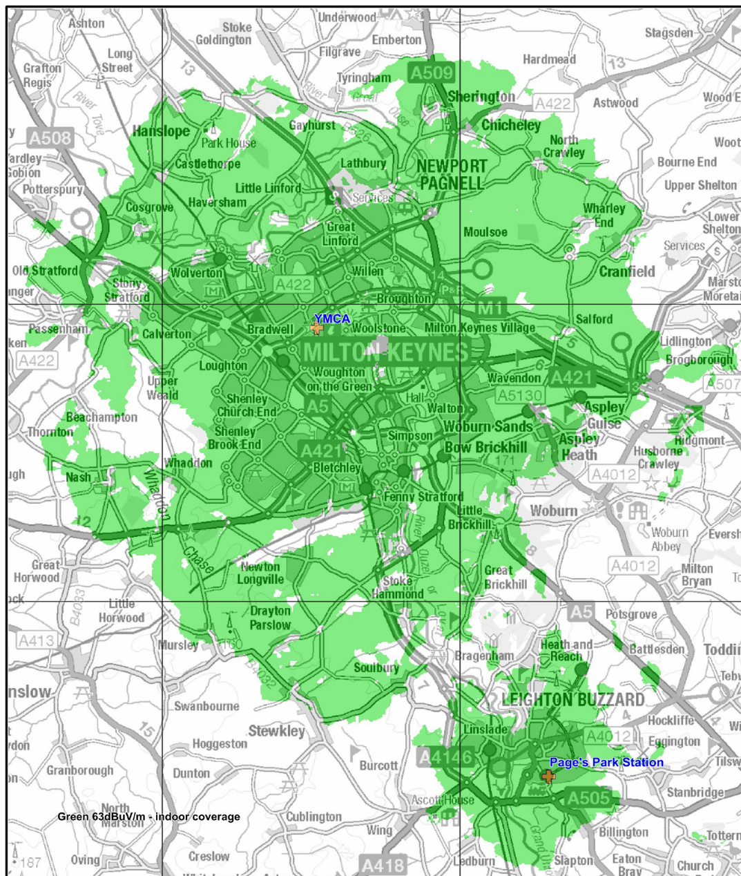
Figure 1: Predicted indoor coverage of the Milton Keynes small-scale DAB multiplex. April 2024.
