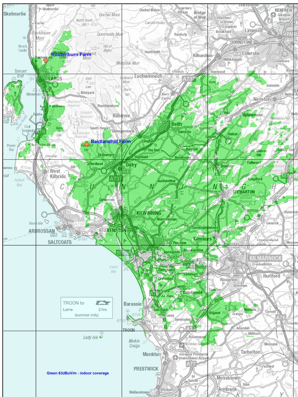
Figure 1: Predicted indoor coverage of the North Ayrshire small-scale DAB multiplex. January 2026
