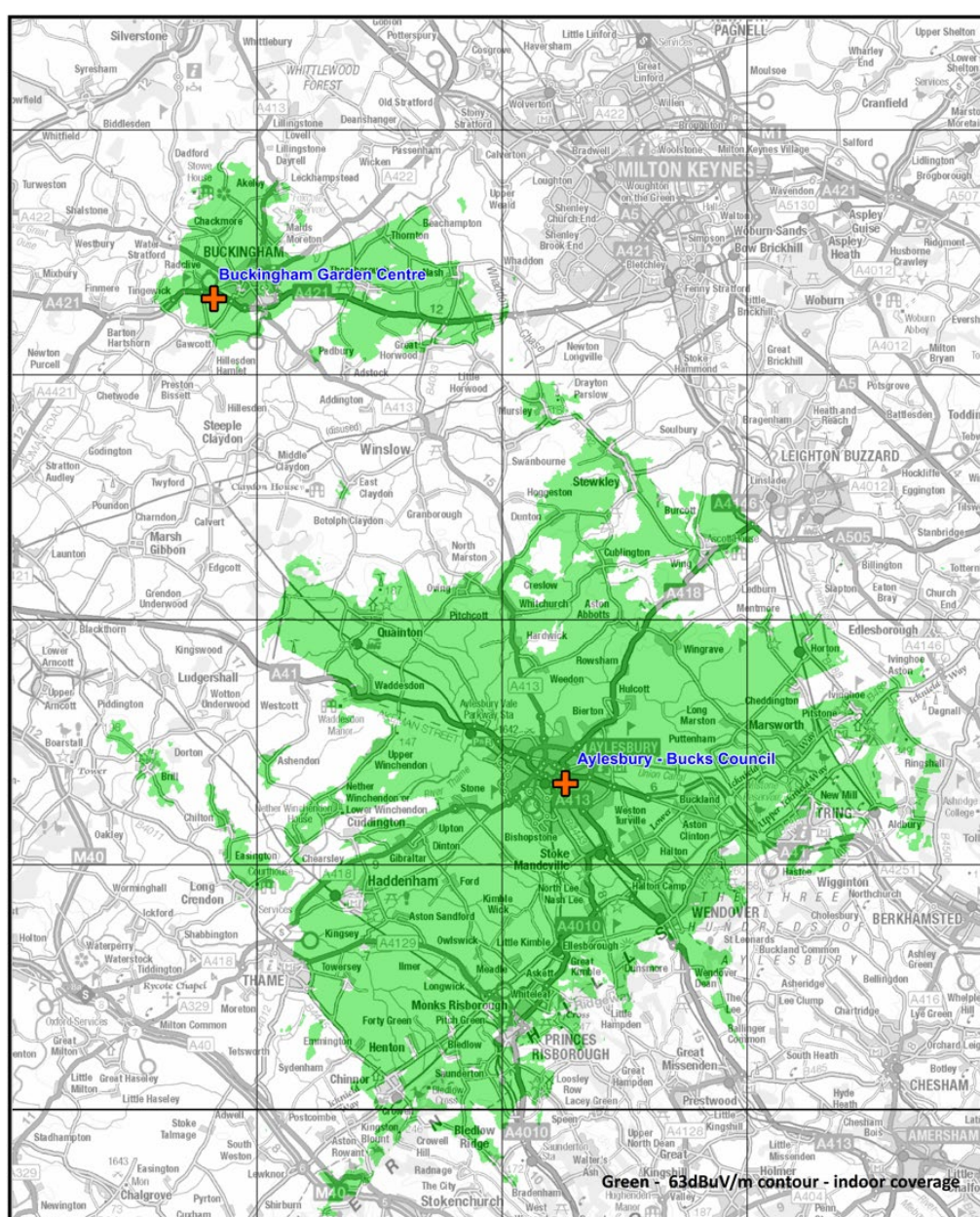
Figure 1: Predicted indoor coverage of the North Buckinghamshire small-scale DAB multiplex. June 2024
