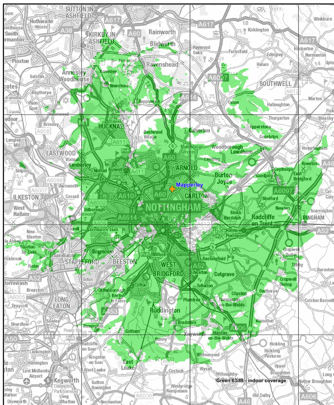
Figure 1: Predicted indoor coverage of the Nottingham small-scale DAB multiplex. January 2024
