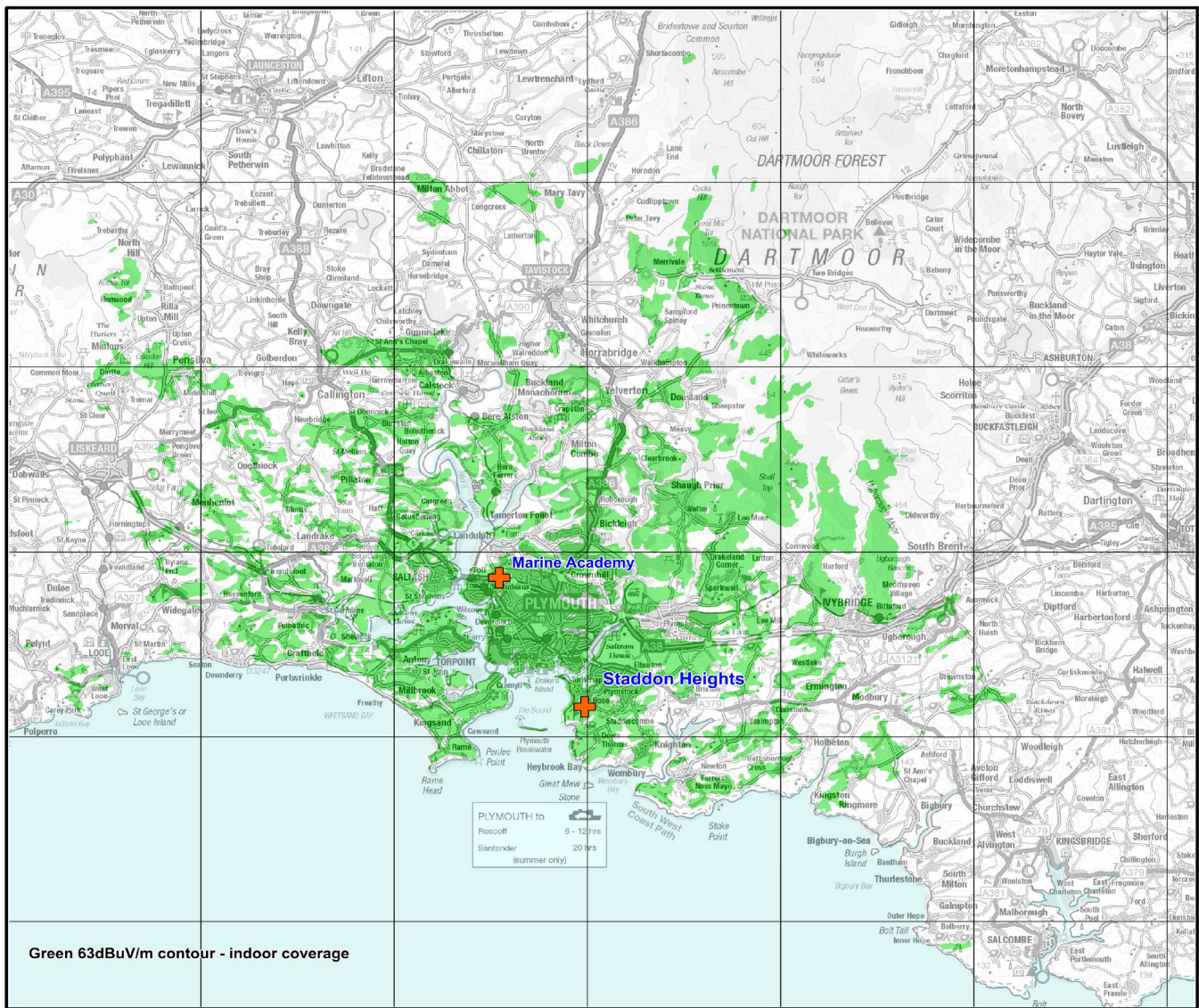
Figure 1: Predicted indoor coverage of the Plymouth small-scale DAB multiplex. July 2023
