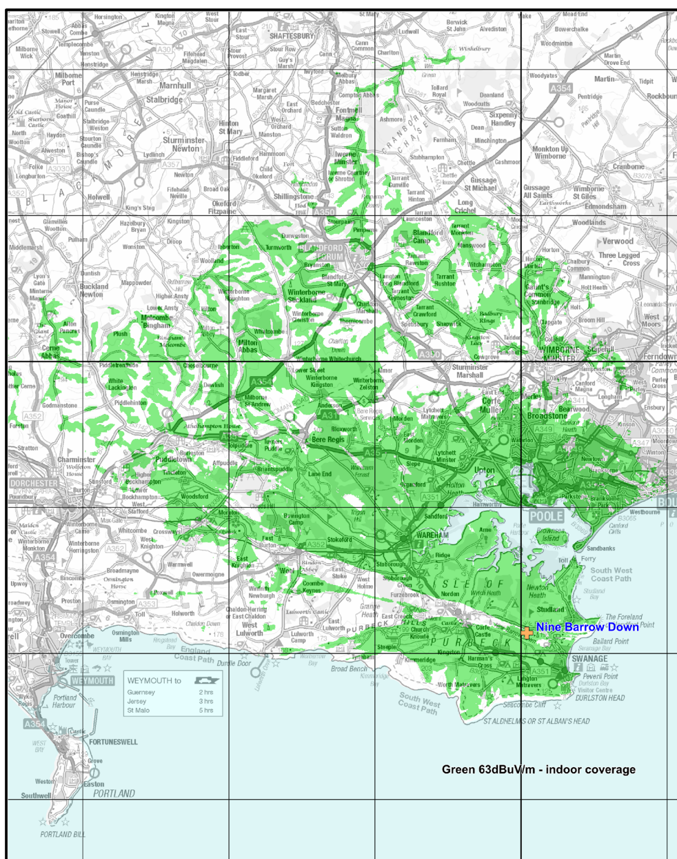
Figure 1: Predicted indoor coverage of the Poole, Purbeck & Wimborne small-scale DAB multiplex. January 2025
