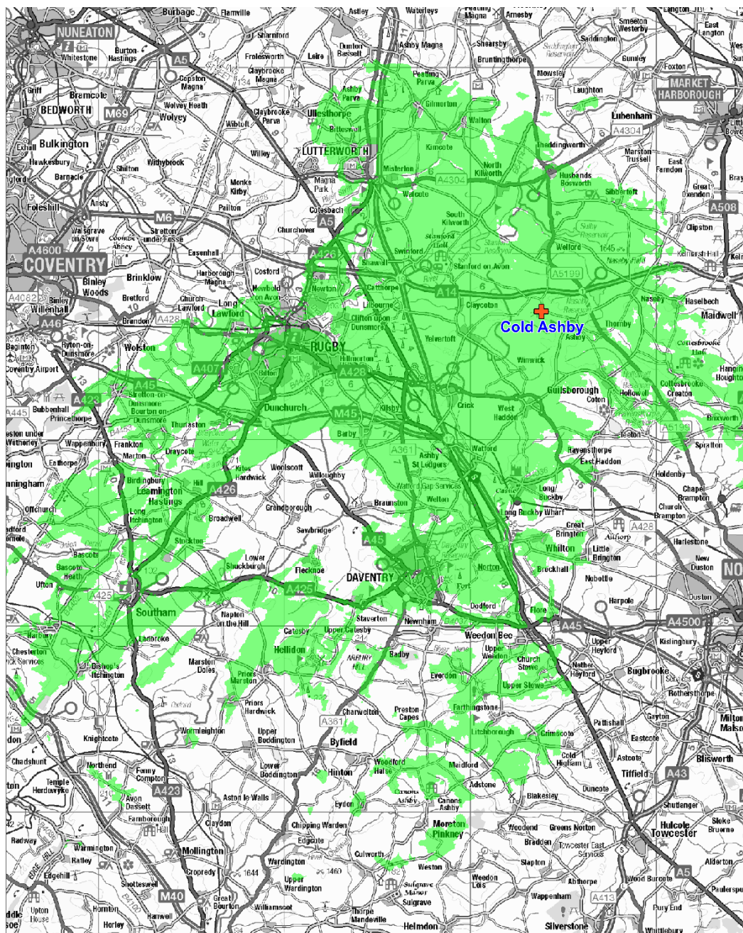
Figure 1: Predicted indoor coverage of the Rugby and Daventry small-scale DAB multiplex. December 2025
