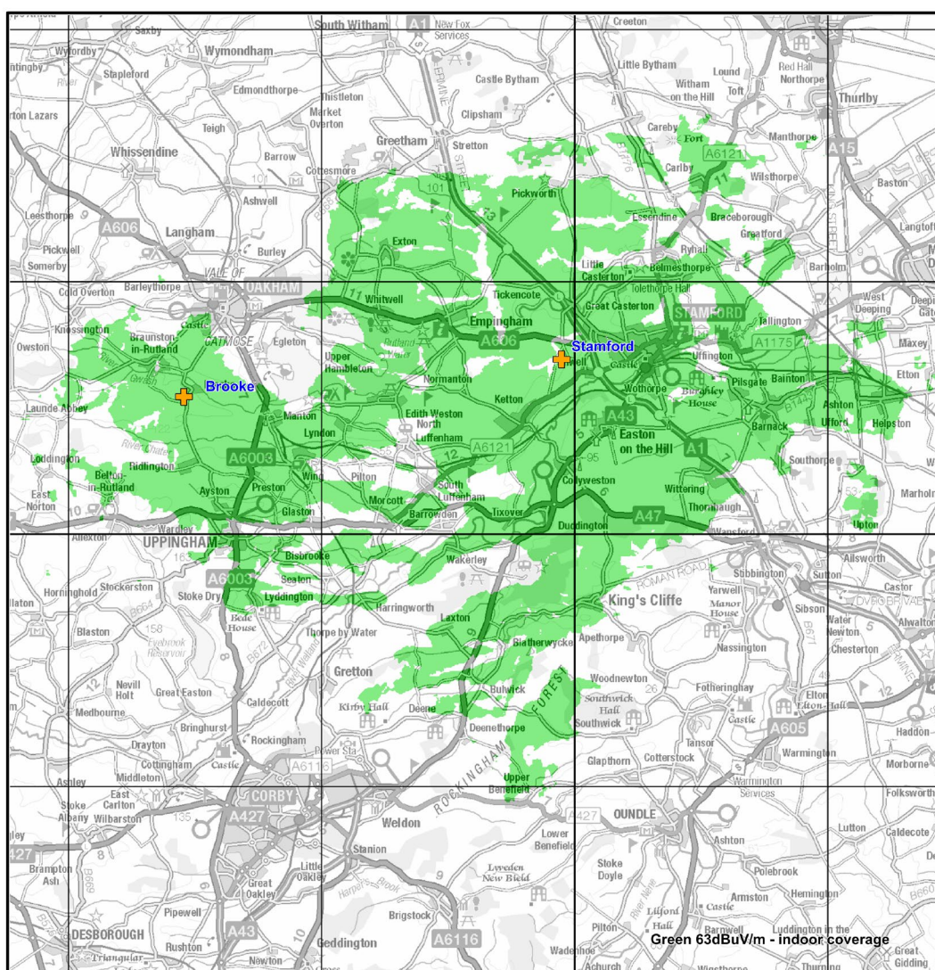
Figure 1: Predicted indoor coverage of the Rutland and Stamford small-scale DAB multiplex. April 2024.
