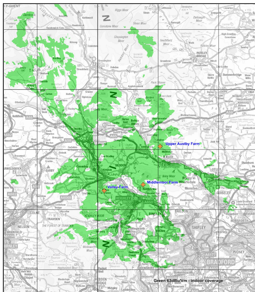
Figure 1: Predicted indoor coverage of the Sout Craven, Wharfedale & Worth Valley small-scale DAB multiplex. May 2026
