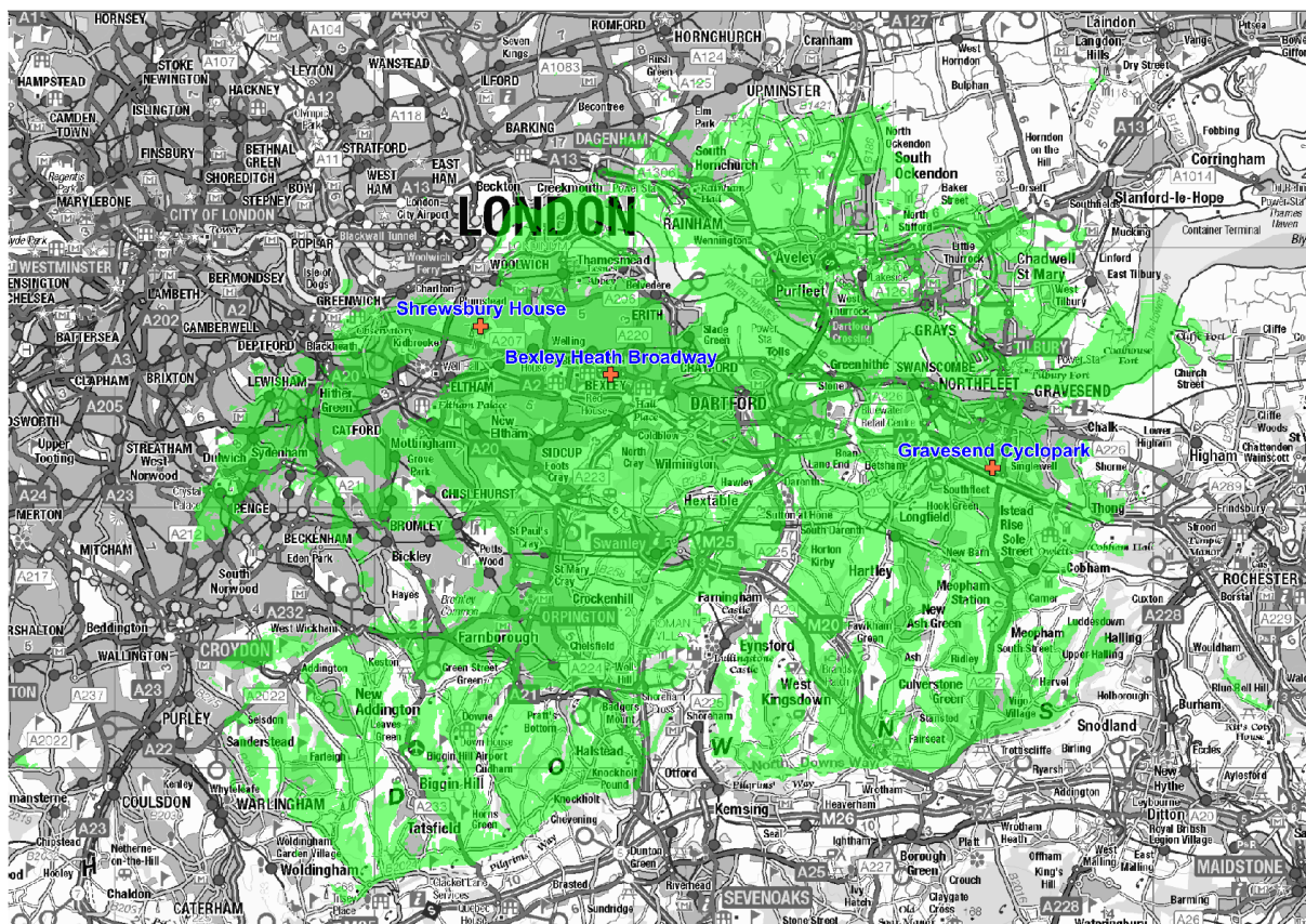
Figure 1: Predicted indoor coverage of the South East London and North West Kent small-scale DAB multiplex. January 2026
