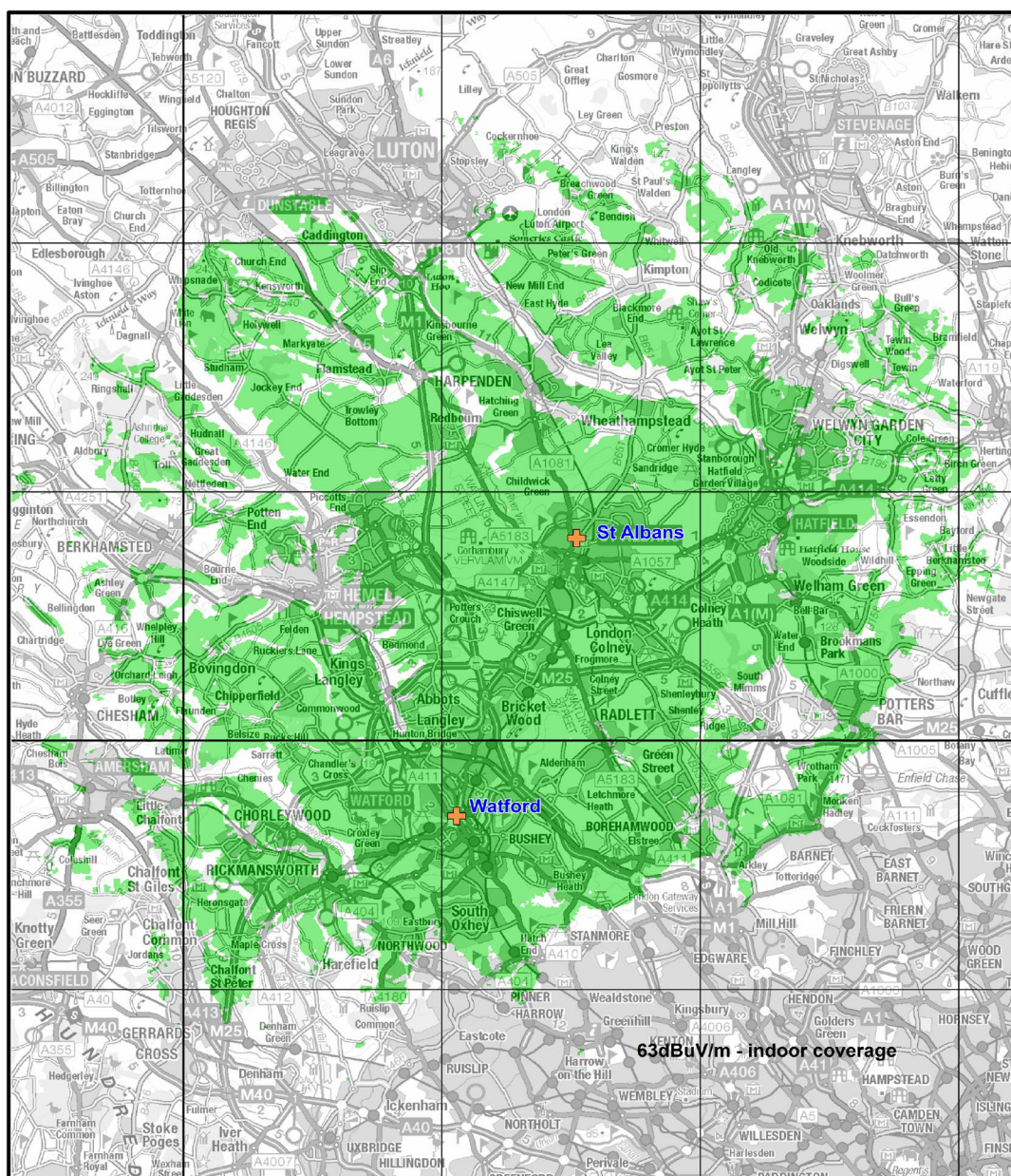
Figure 1: Predicted indoor coverage of the South Hertfordshire small-scale DAB multiplex. January 2025.
