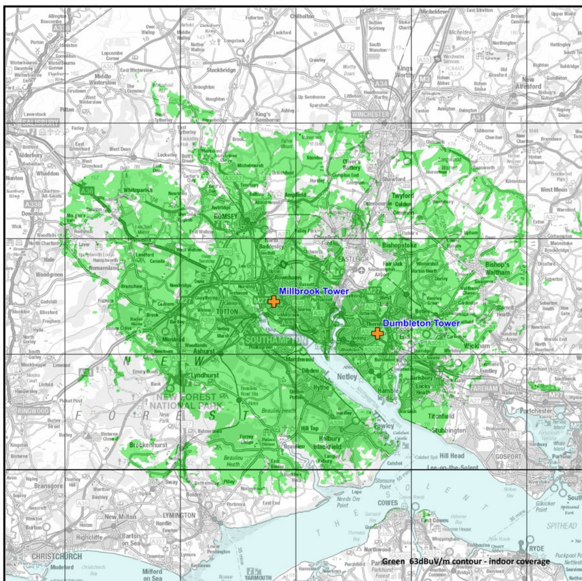
Figure 1: Predicted indoor coverage of the Southampton small-scale DAB multiplex. August 2024
