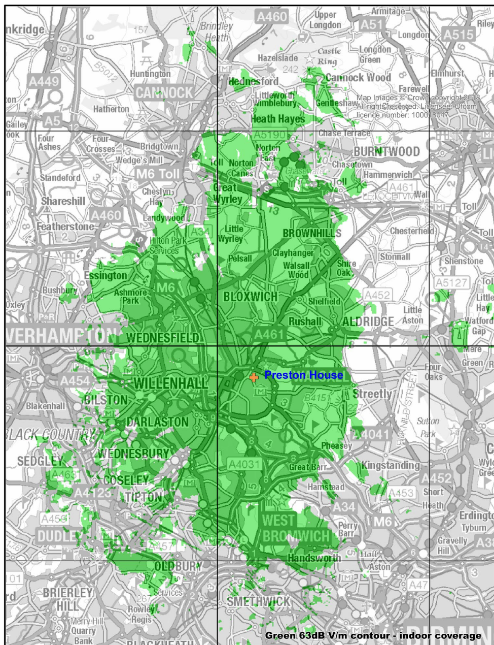
Figure 1: Predicted indoor coverage of the Walsall DAB multiplex. October 2025.
