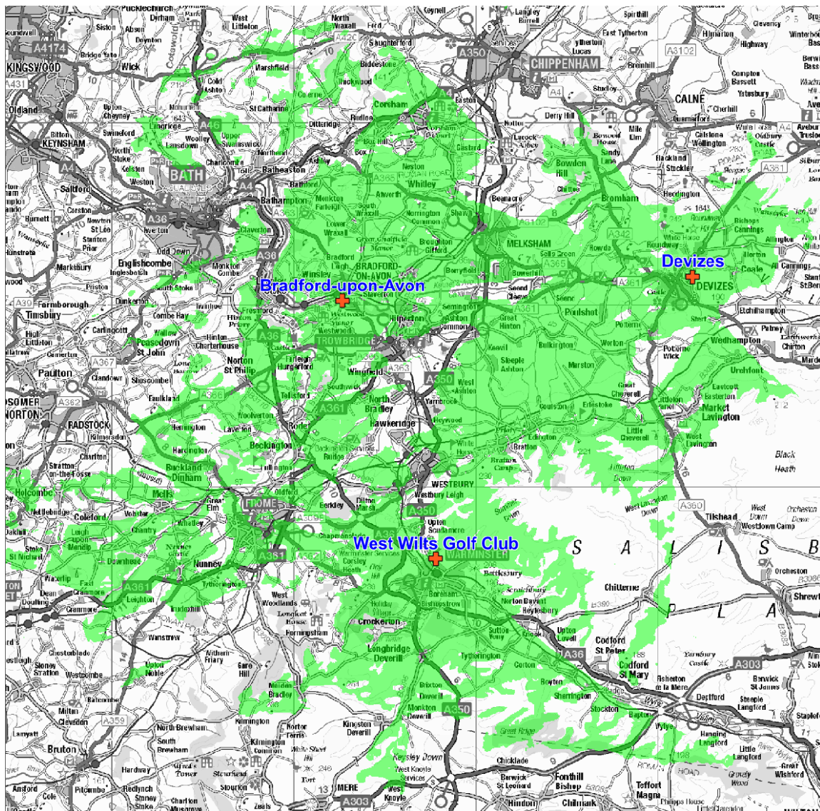
Figure 1: Predicted indoor coverage of the Warminster Devizes and Trowbridge small-scale DAB multiplex. April 2026
