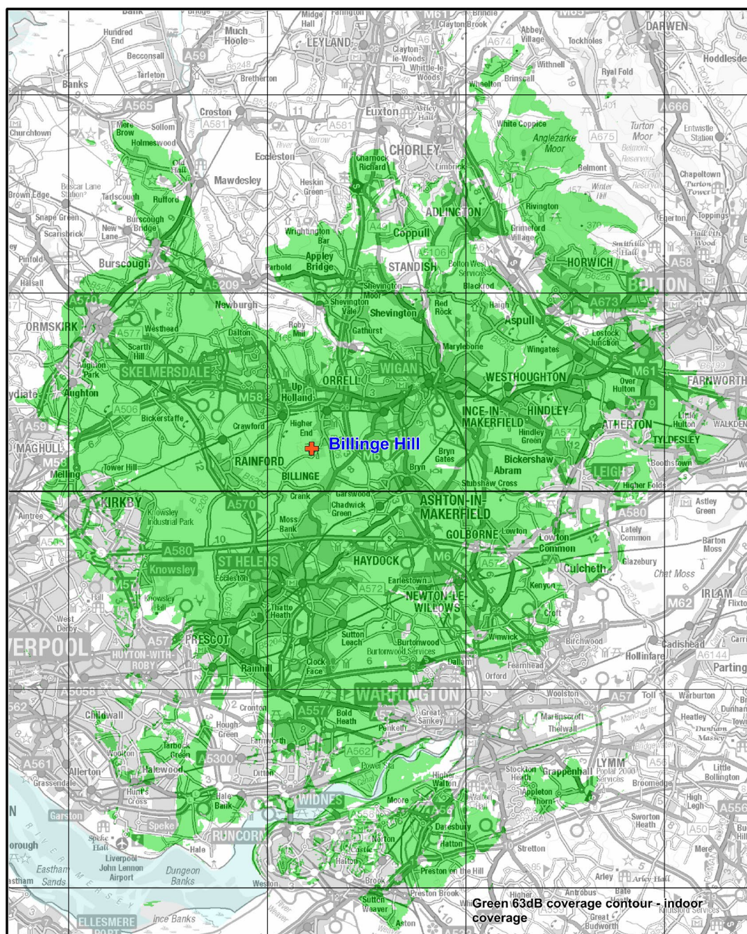
Figure 1: Predicted indoor coverage of the Wigan small-scale DAB multiplex. May 2026
